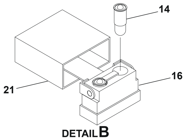
ANNUNCIATOR PANEL INSTALLATION Figure 02. (Sheet 1)
