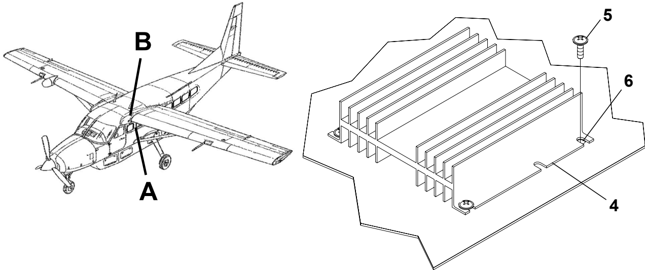
DETAIL A
