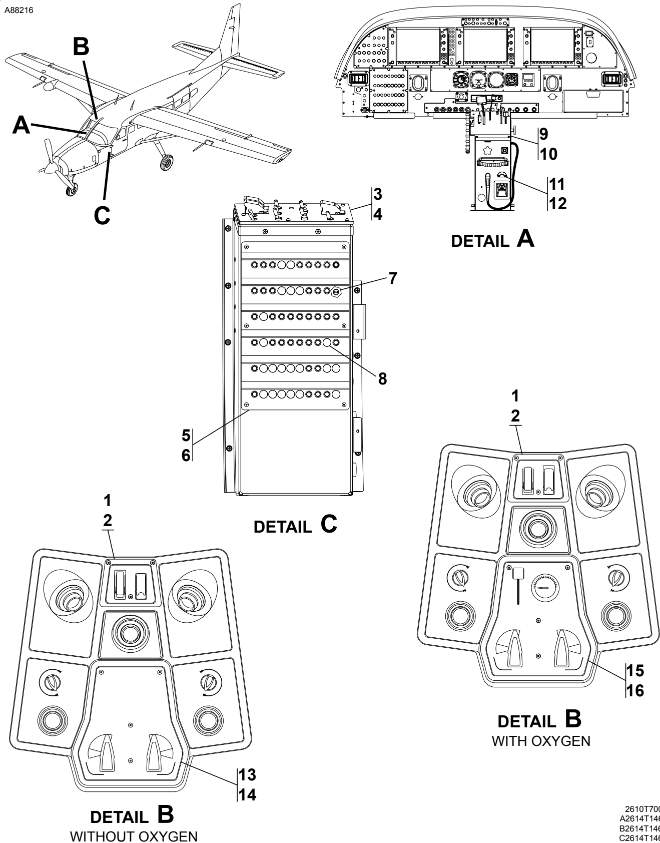
LED PANELS Figure 01. (Sheet 1)
