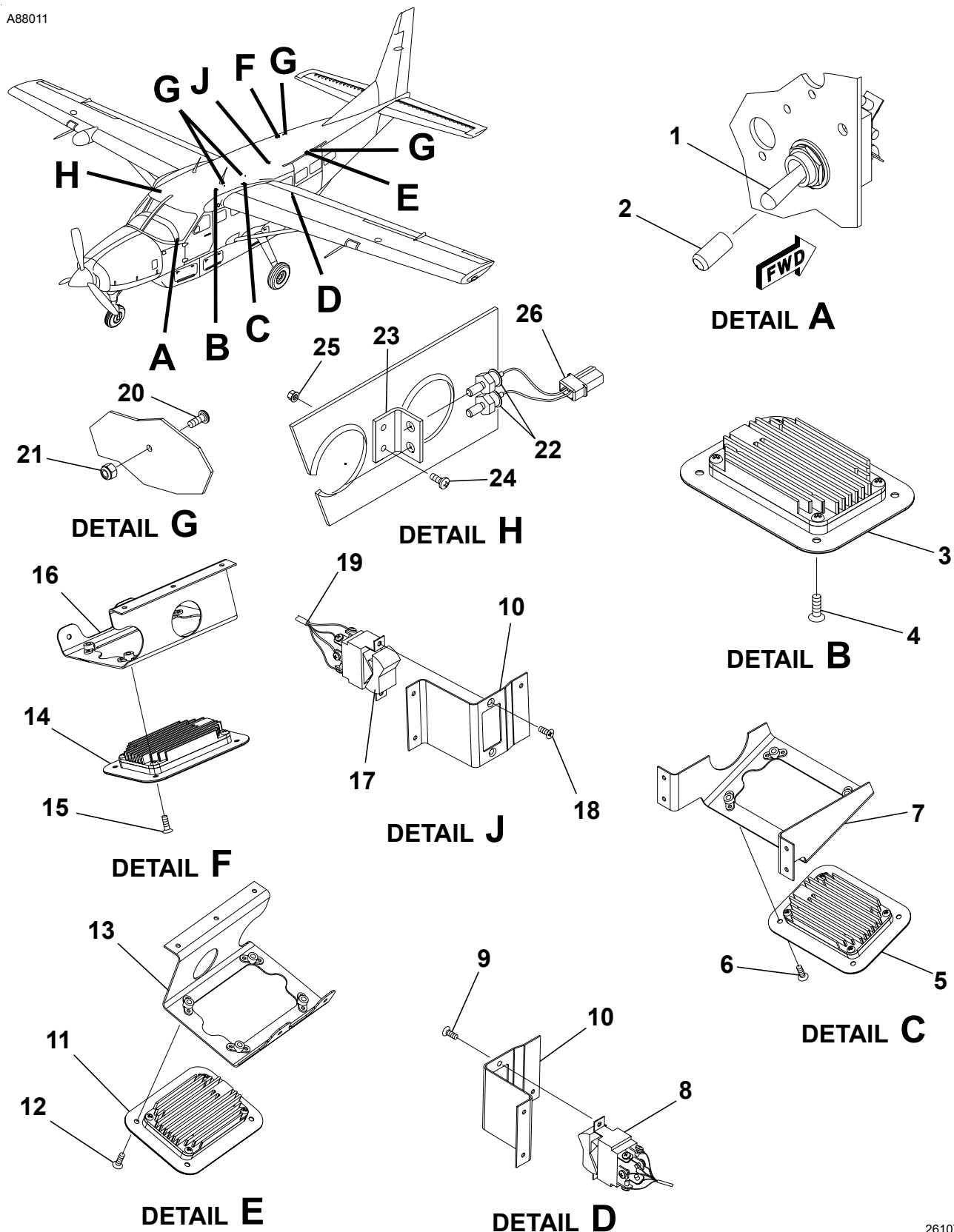
CABIN LIGHTING INSTALLATION Figure 01A. (Sheet 1)
