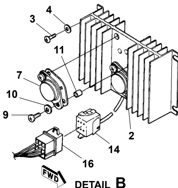
INSTRUMENT PANEL LIGHTING INSTALLATION Figure 01. (Sheet 1)
