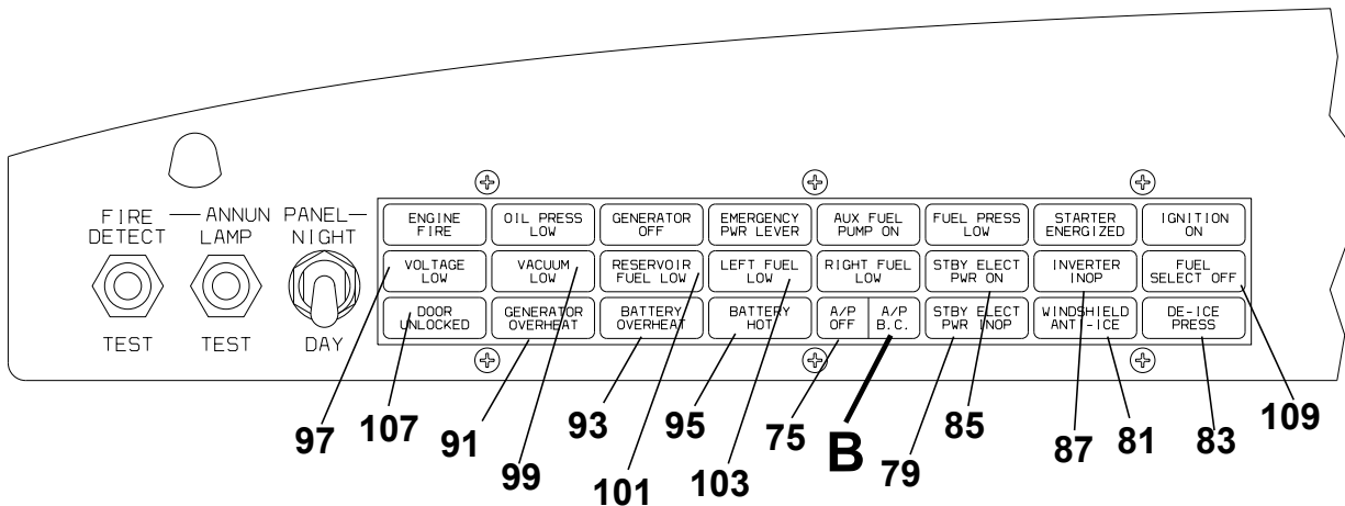
DETAIL A
