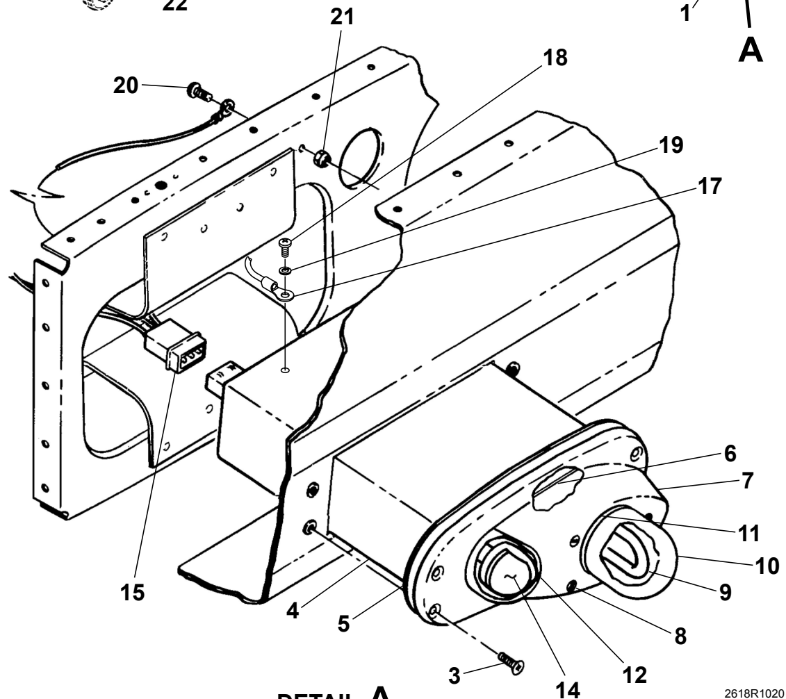
DETAIL A WING NAVIGATION AND STROBE LIGHT INSTALLATION Figure 01. (Sheet 1)
