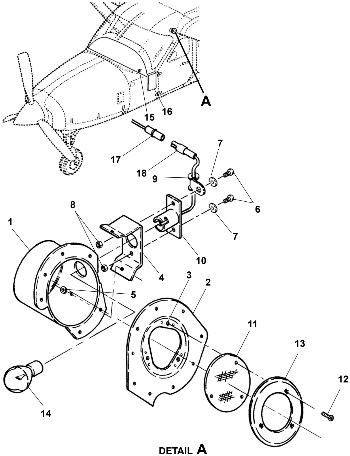
ICE DETECTOR LIGHT INSTALLATION Figure 01. (Sheet 1)
